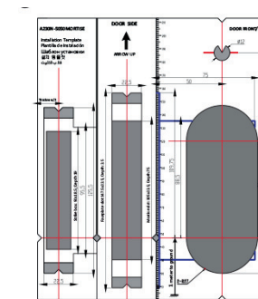
Drill Hole with Template
